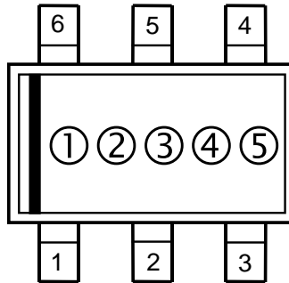
SOT-23-6W Part Markings
